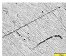
Sharp angles, rings and strange tracks (Savvatimova, Matsumoto, Shoulders)
