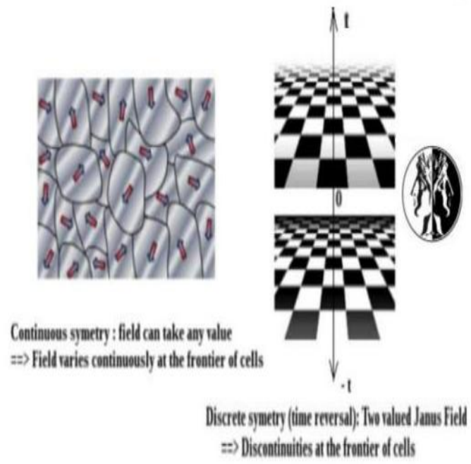
Fig. 3. Discrete symmetry domains vs continuous symmetry breaking domains
