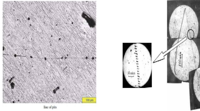
Line of pits and caterpillar tracks (Savvatimova, Unutskoev)
