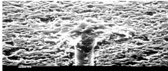
Fig. 4 Entrance cross section of EV borehole in aluminum oxide showing sloshing cycles.
