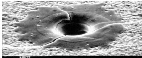
Fig. 6 SEM micrograph of EV entrance into lead glass showing wave action of sloshing.
