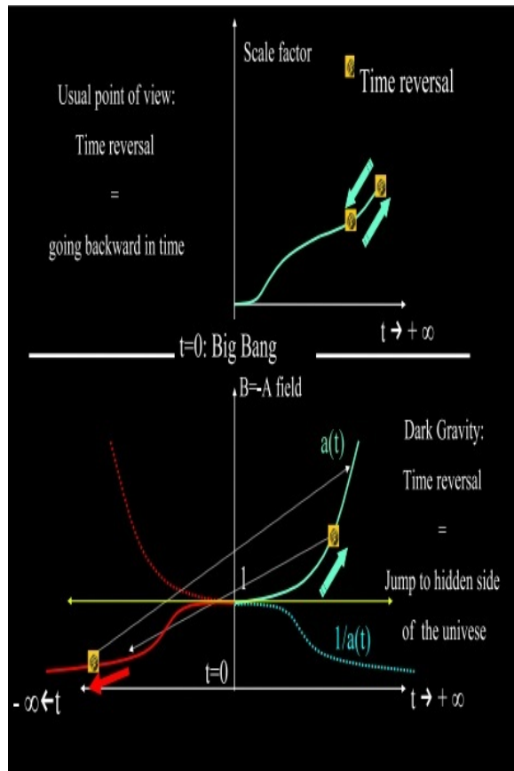
Fig. 1. Time reversal in DG vs RG, plotted curves are not realistic
